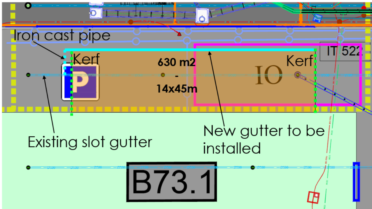
Figure 6 – Schema of the gutter system to be installed
